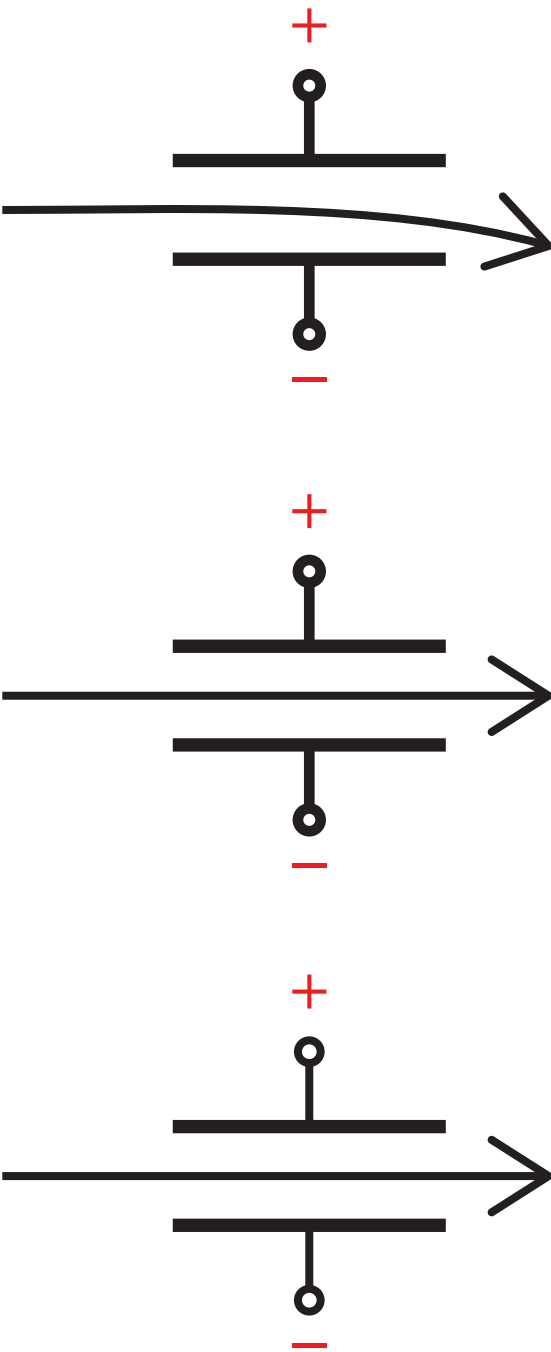
Path taken by gamma radiation
