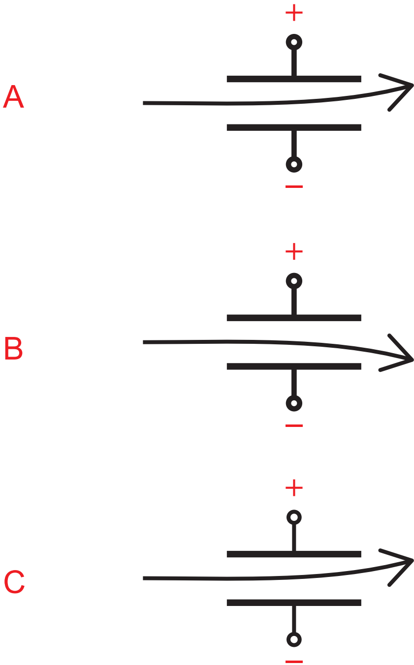
Path taken by alpha particles
