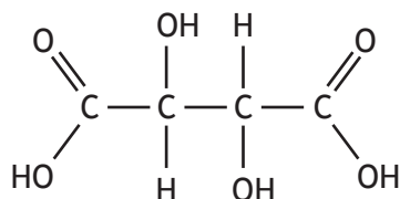
tartaric acid
