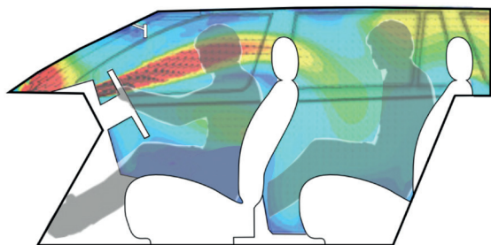
CFD test of a ventilation system
