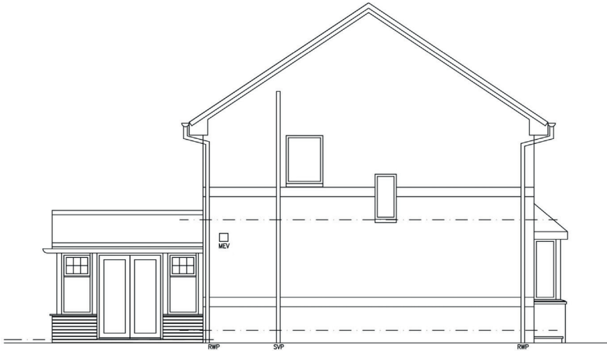
SIDE ELEVATION AS EXISTING
