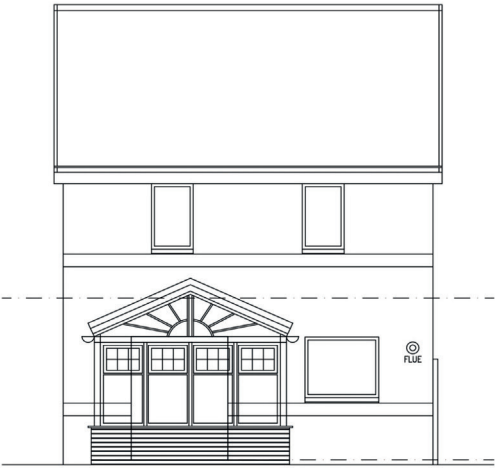
REAR ELEVATION AS EXISTING
