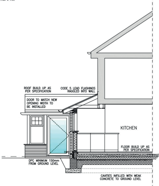
SECTION A-A AS PROPOSED
