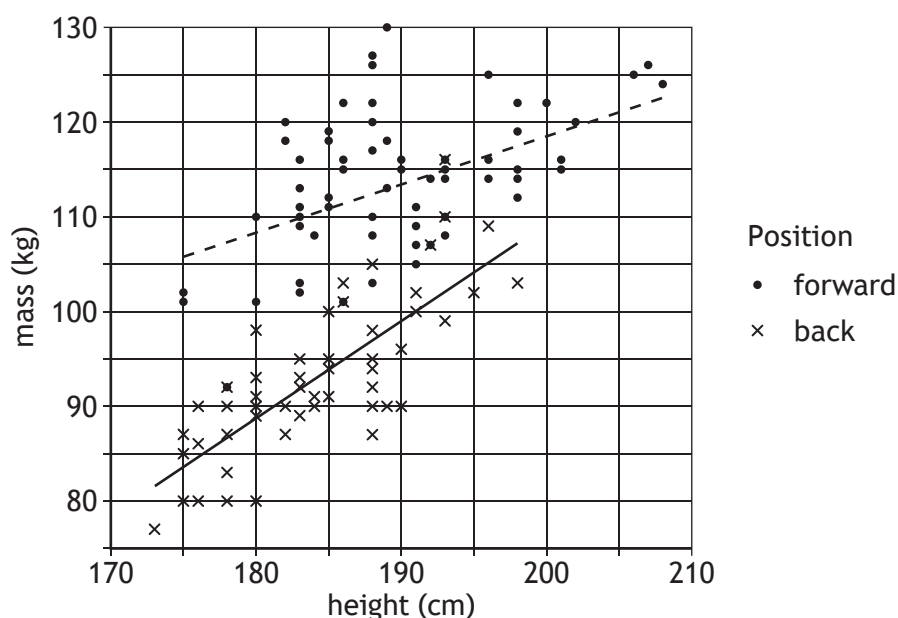
Figure 1 Scatterplot of masses and heights of players, their playing positions identified, and the associated least squares regression models
