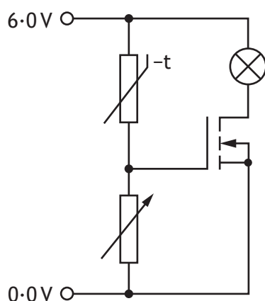
Circuit A
