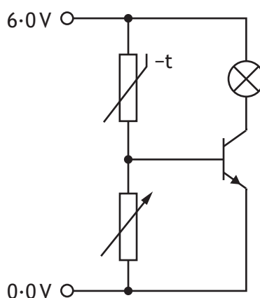
Circuit B
